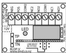
Remove Link from RLDP-V
