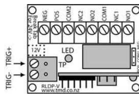
RLDP-CB1 and Connector Installed on RLDP-V
